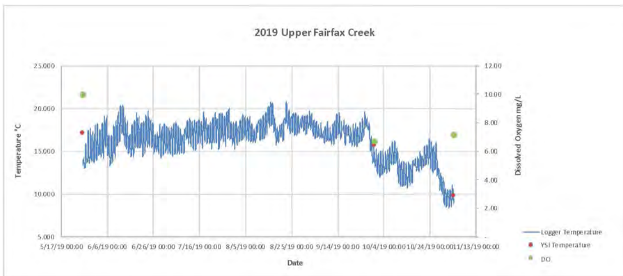
Figure 9: Temperature and DO in Fairfax Creek downstream of 300 Olema Road
