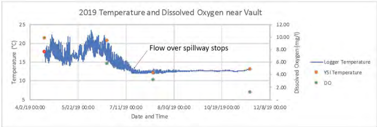
Figure 4: Temperature and DO in Ross Creek near Vault
