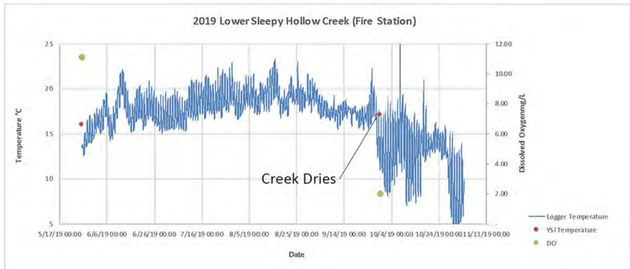
Figure 14: Temperature and DO in Sleepy Hollow Creek at Fire Station
