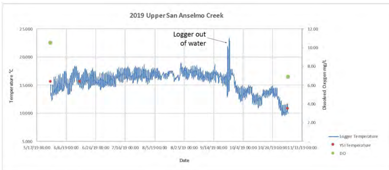
Figure 11: Temperature and DO in San Anselmo Creek near Deer Park Creek
