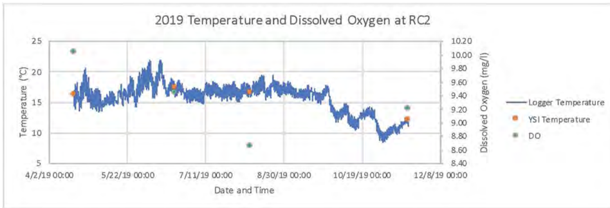
Figure 7: Temperature and DO in Ross Creek at Logger RC2
