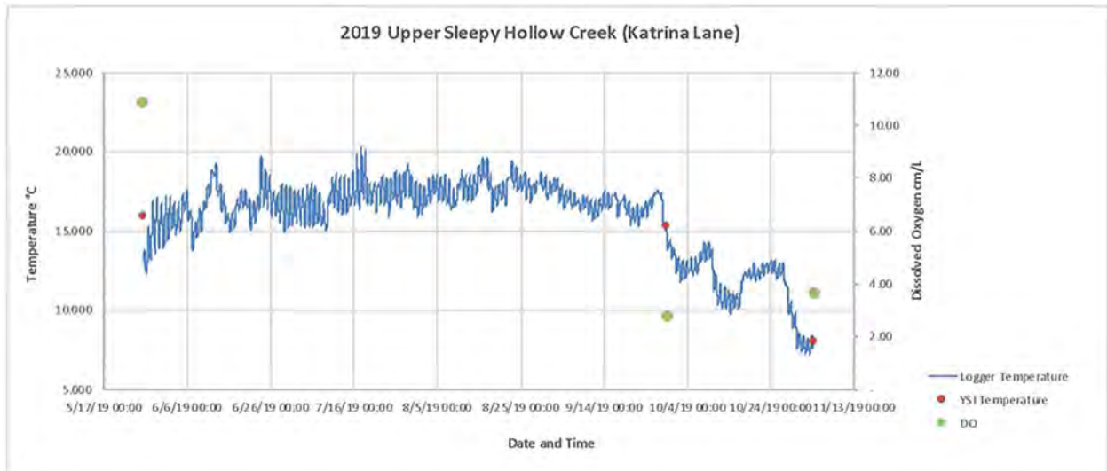
Figure 13: Temperature and DO in Sleepy Hollow Creek at Katrina Lane
