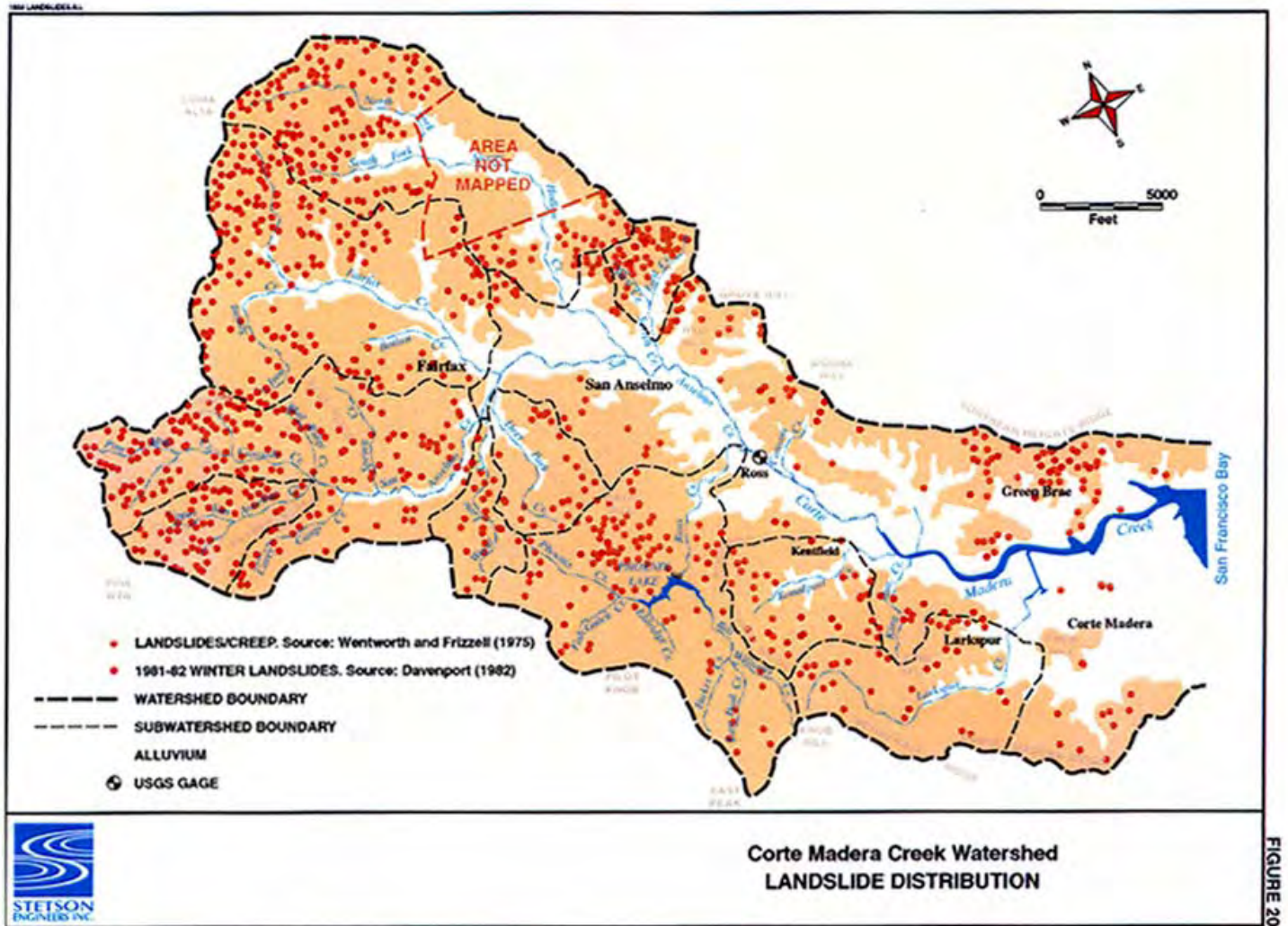
Figure 20 Landslide distribution
