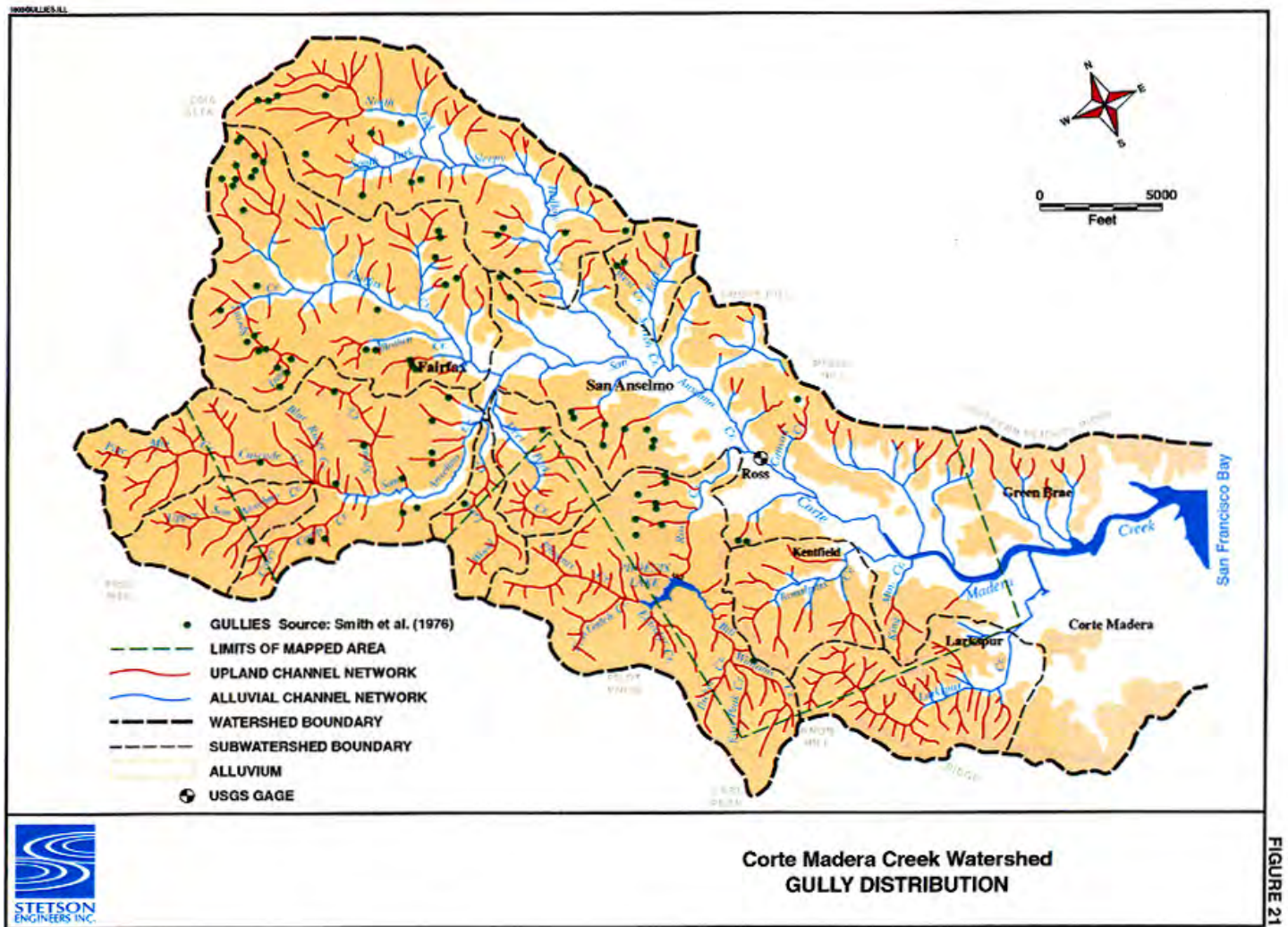
Figure 21 Gully distribution
