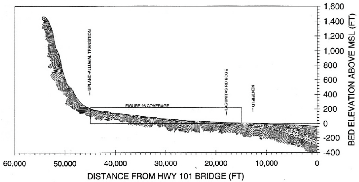
Figure 9 Longitudinal profile of the mainstem Corte Madera - San Anselmo Creek
