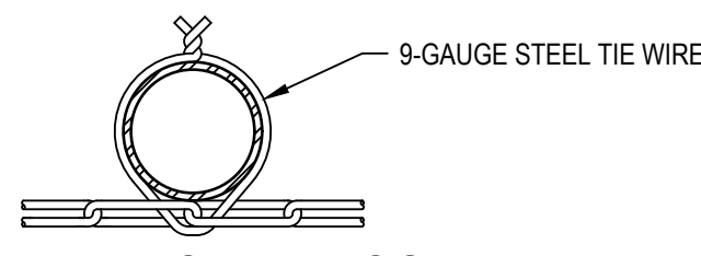
PLAN - ROUND POST
