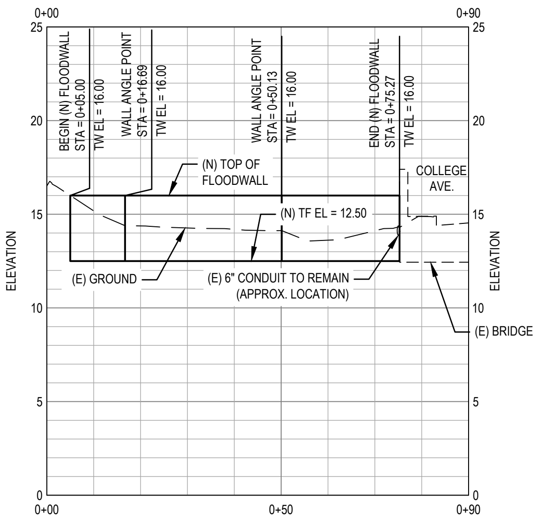
PROFILE - FREE STANDING FLOOD WALL
