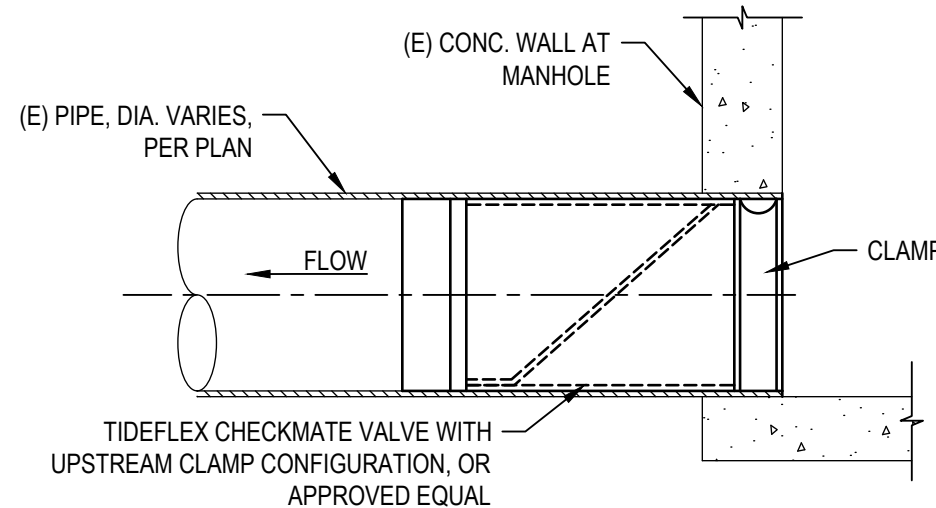
6 IN-LINE CHECK VALVE - UPSTREAM CLAMP NOT TO SCALE
