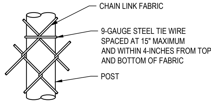
ELEVATION - ROUND POST
