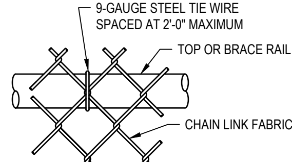
TOP OR BRACE RAIL ATTACHMENT
