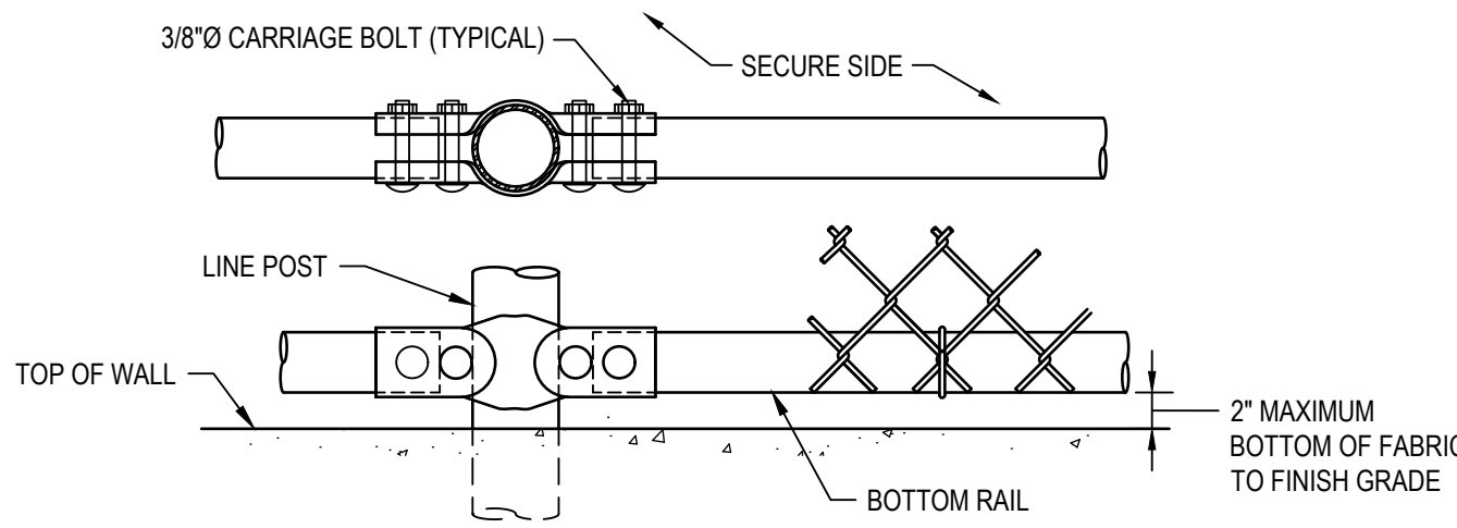
BOTTOM RAIL OPTION
