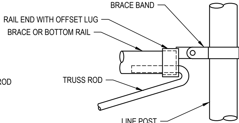
ELEVATION - ROUND POST
