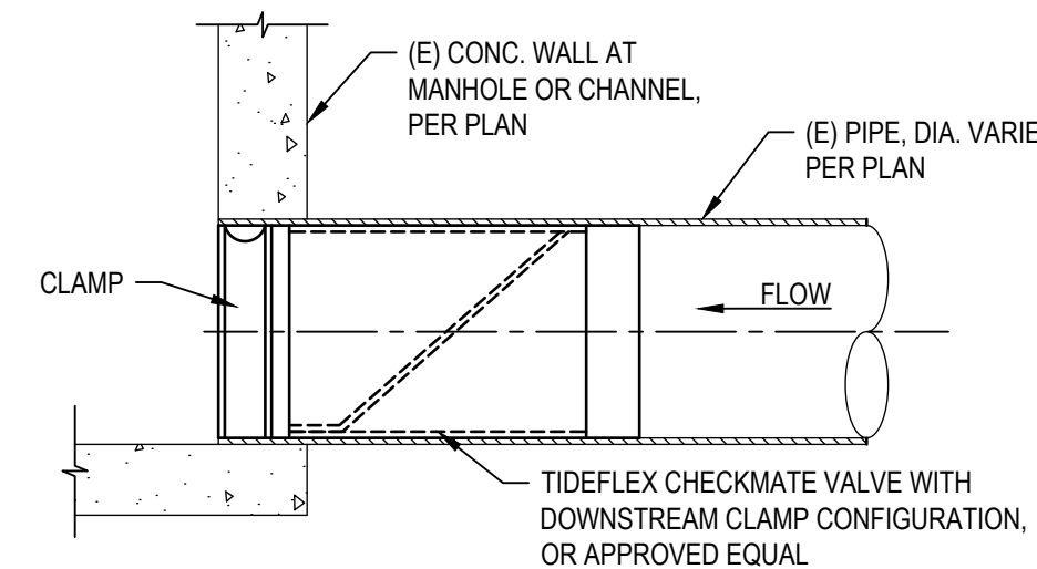
5 IN-LINE CHECK VALVE - DOWNSTREAM CLAMP NOT TO SCALE
