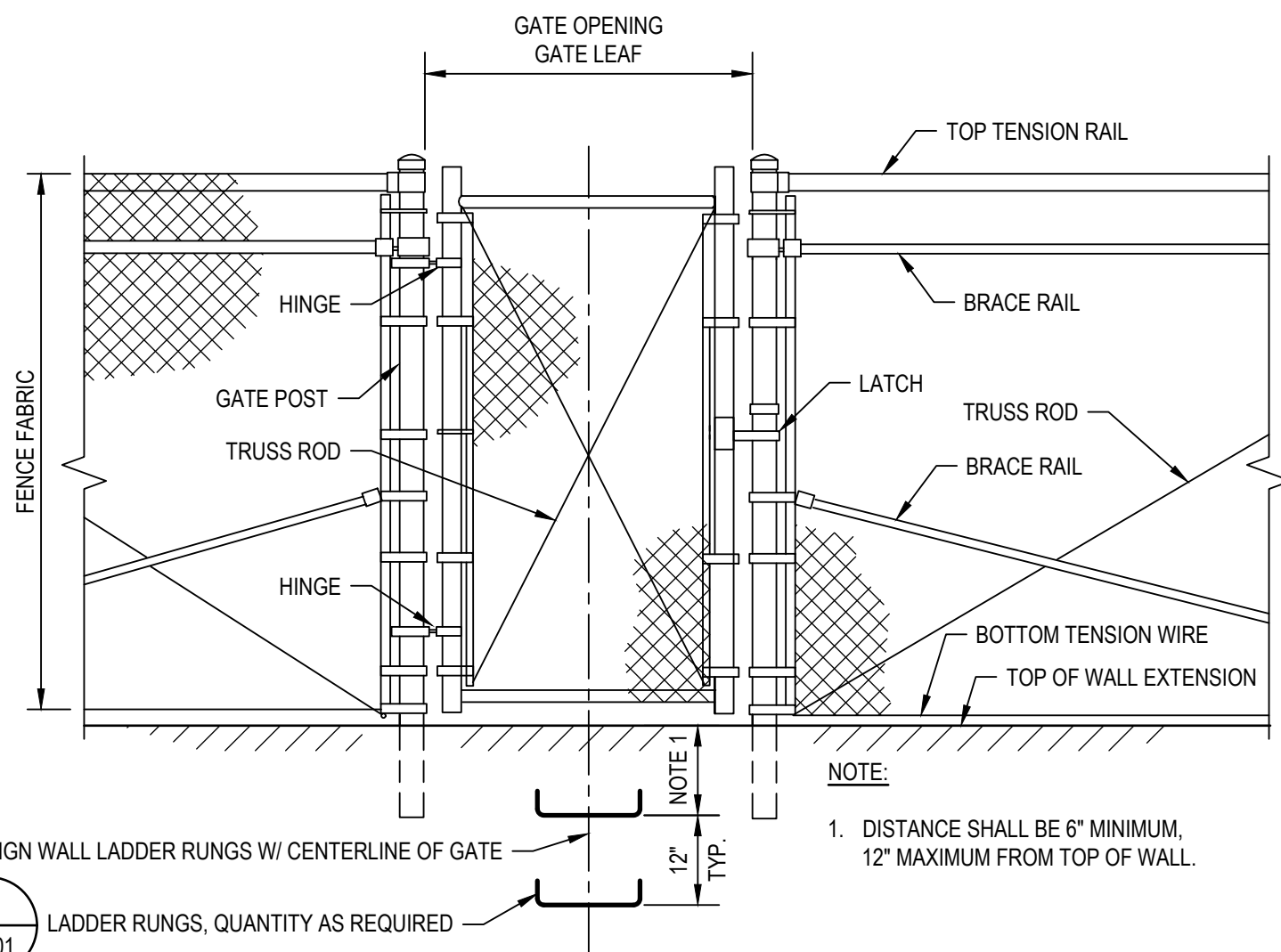
2 PERSONNEL GATE NOT TO SCALE
