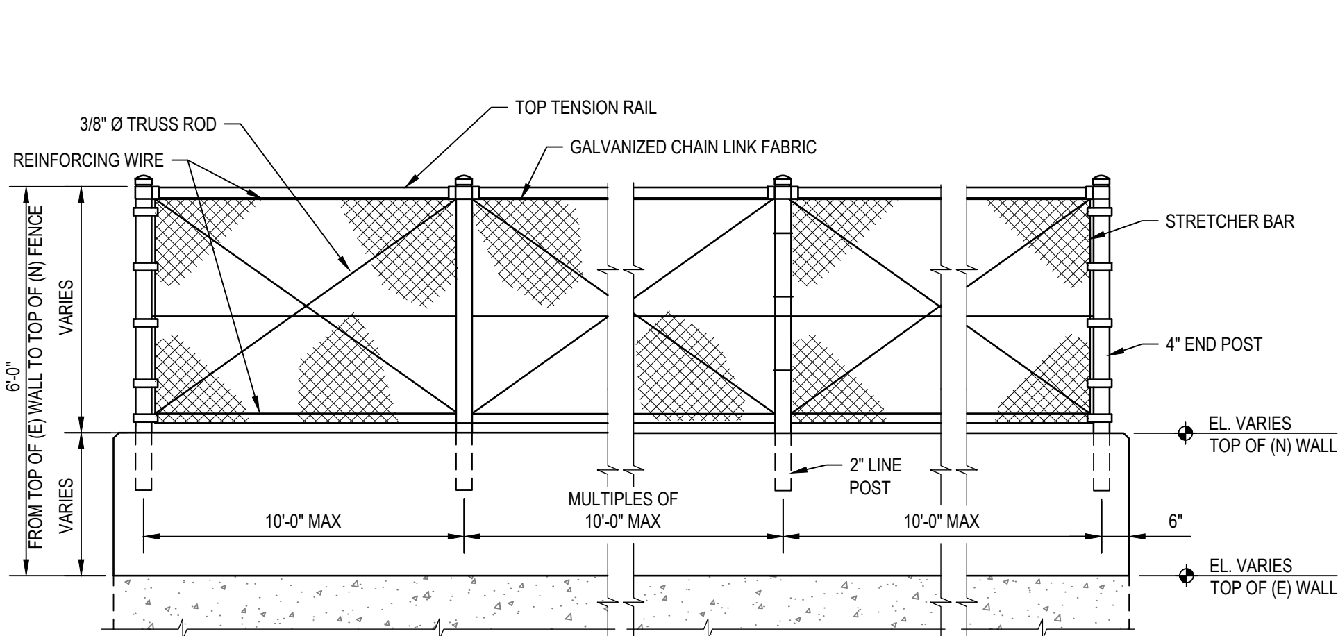
1 CHAIN LINK FENCE ELEVATOIN NOT TO SCALE
