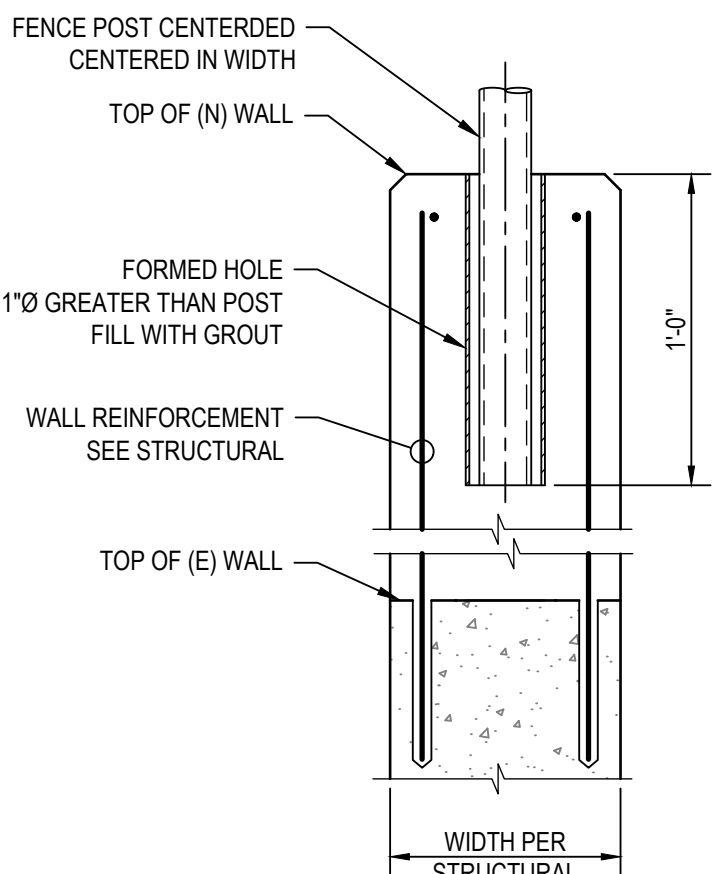
POST BASE CONNECTION
