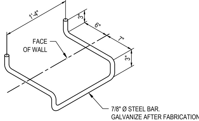
7 WALL LADDER RUNG NOT TO SCALE
